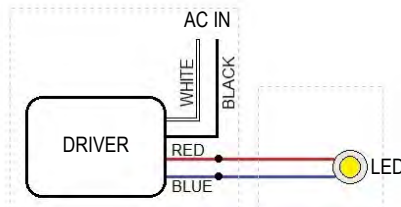
ELV / TRIAC Driver Block Diagram
